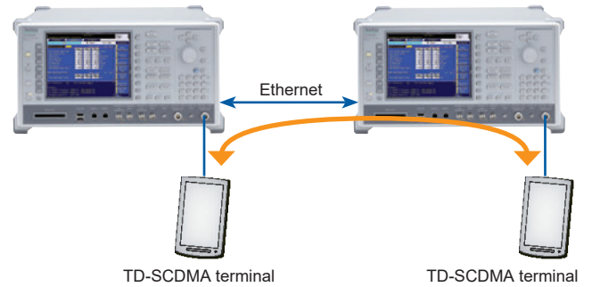
End-to-end Videophone Test Setup using Two MT8820C units
